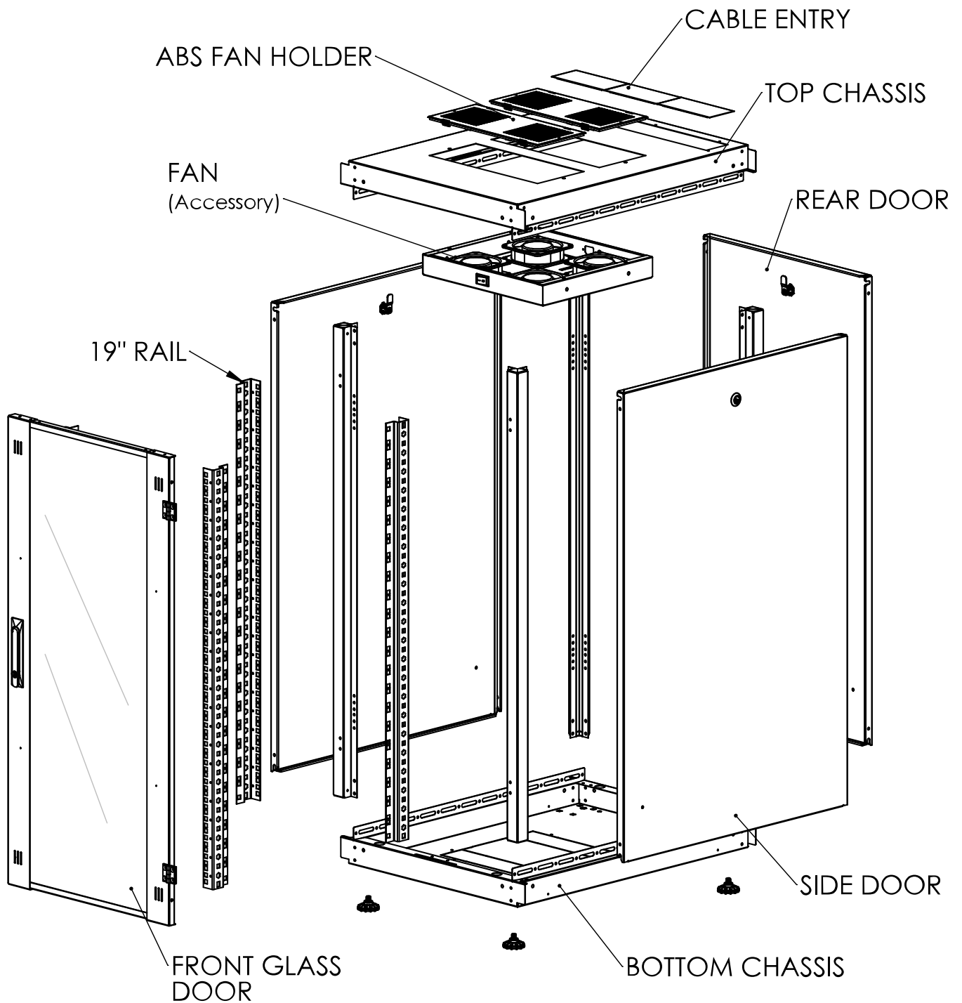
Exploded view
