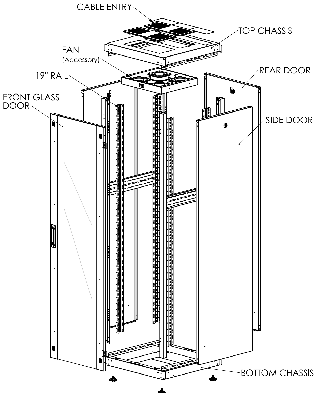
Exploded view
