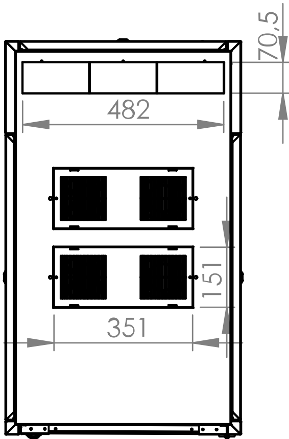
Top view
