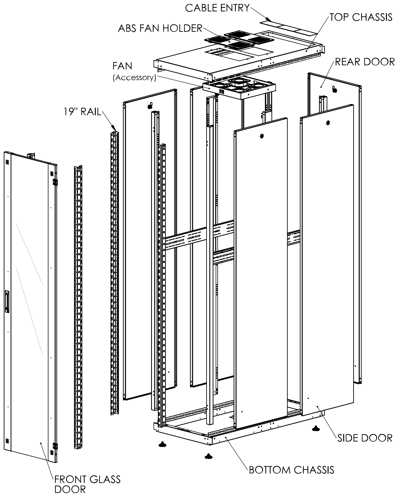
Exploded view
