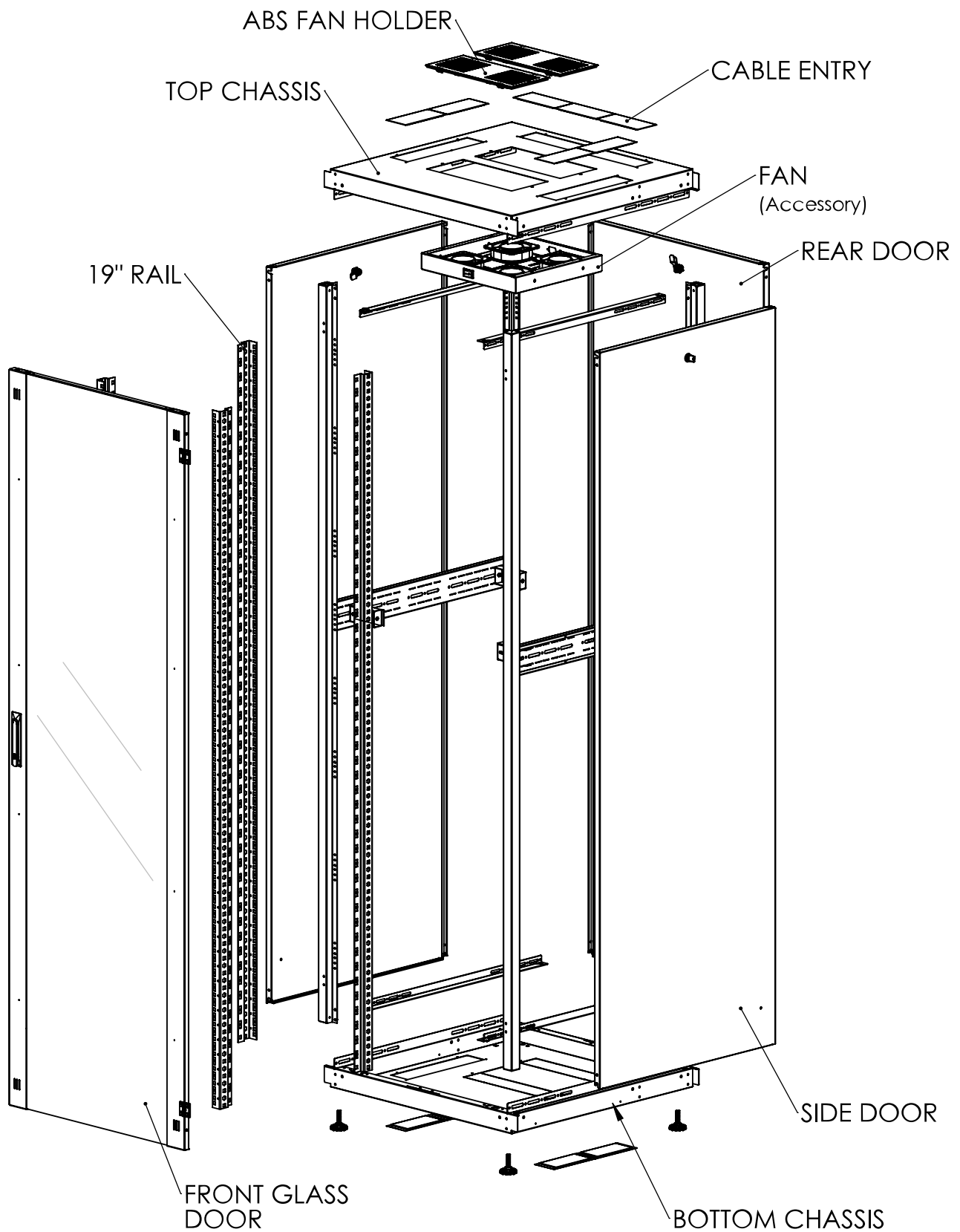
Exploded view
