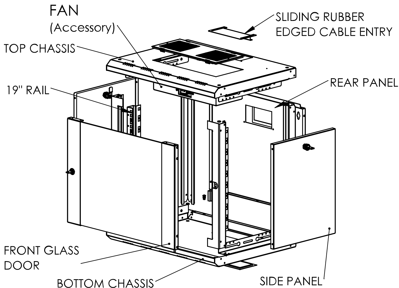
Exploded view
