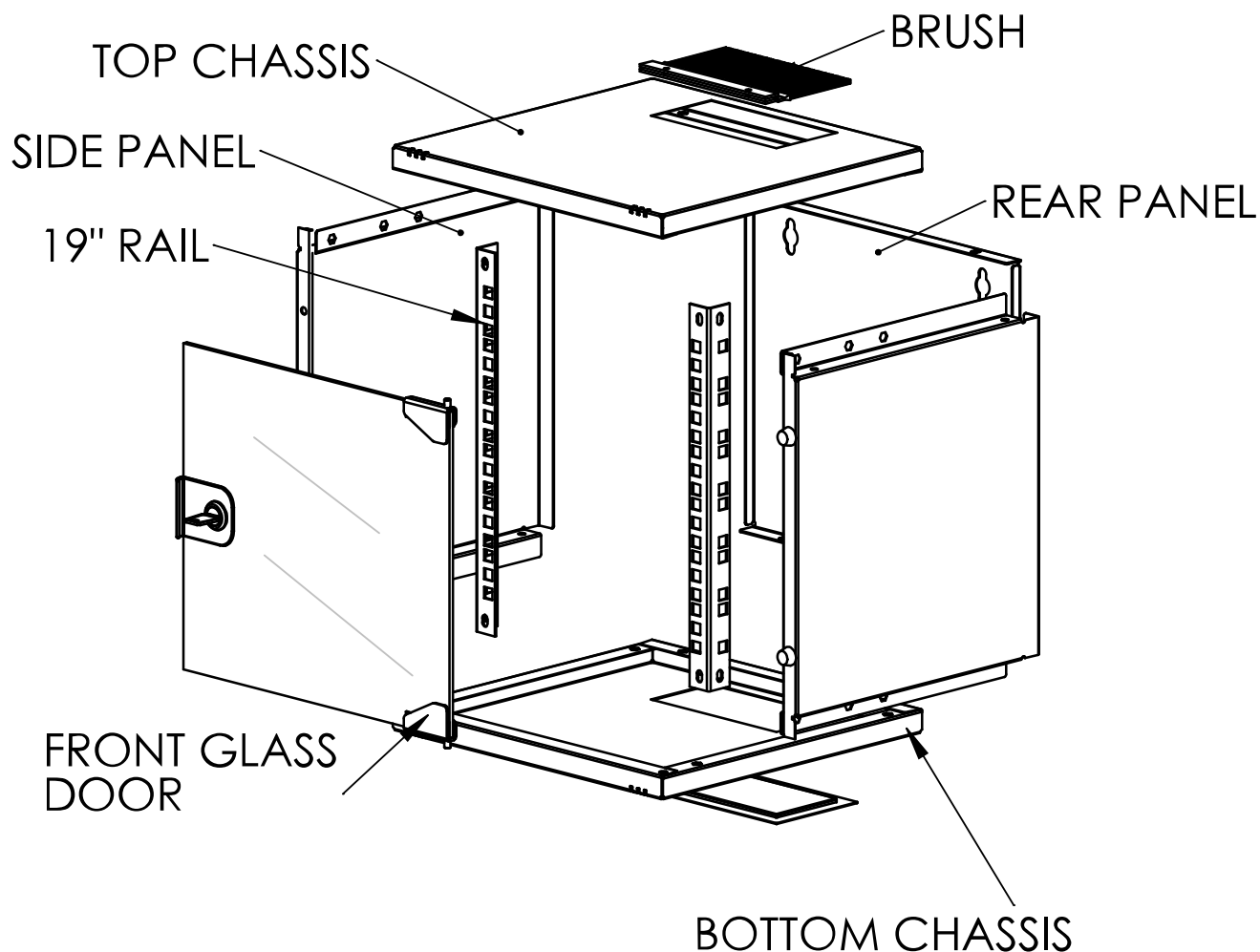
Exploded view
